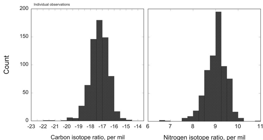
Fig. 2. Frequency distributions of scalp hair carbon and nitrogen isotope ratios across the United States.
