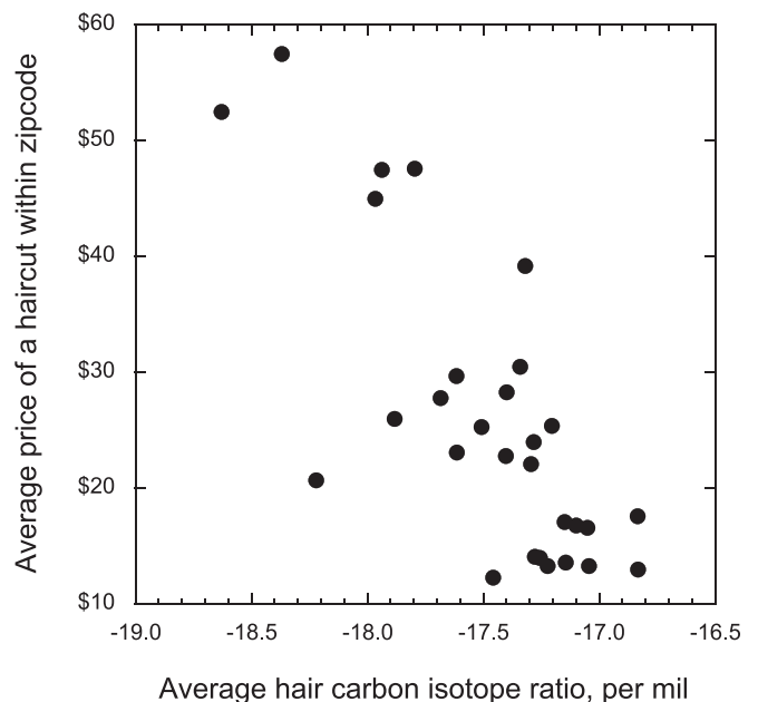
Fig. 5. A plot of the correlation between average carbon isotope ratio of human scalp hair and the average cost of a haircut in ZIP codes within the SLV ( r = -0.767 , n = 29 ; P < 0.001 ).
